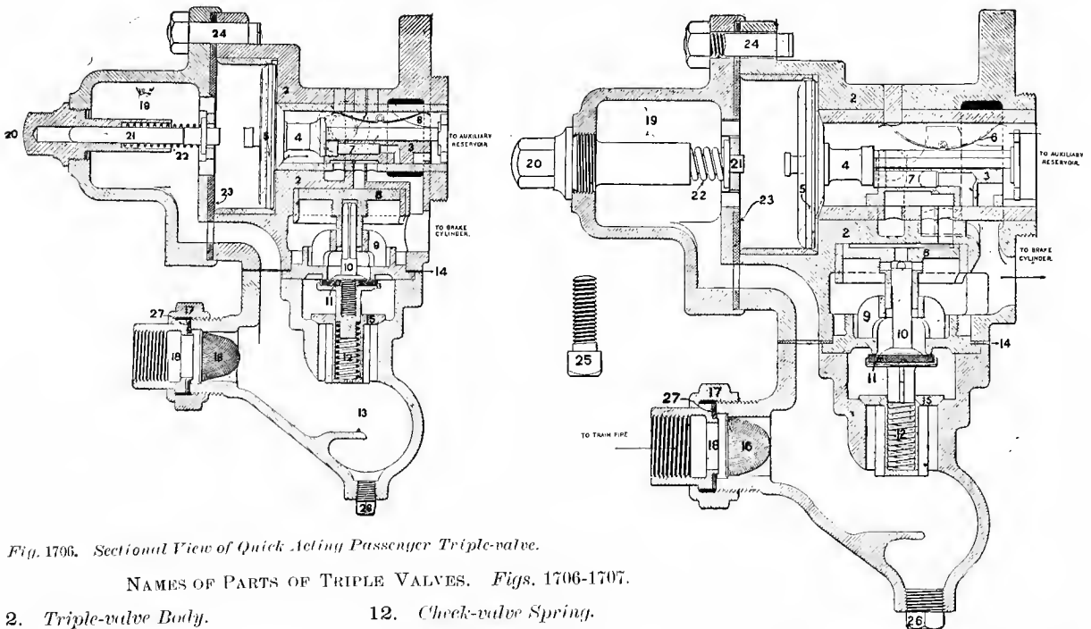
Fig. 1707. Sectional View of Special Quick Acting Passenger Triple-valve.
